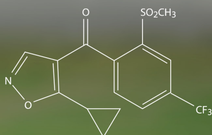
Isoxaflutole → Diketonitrile → Ac. Benzóico
